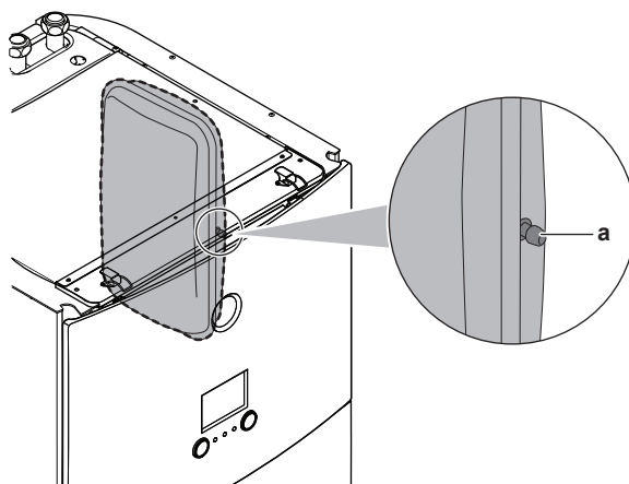
a Valvola Schröder
