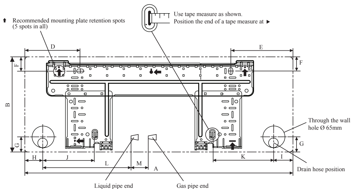
INSTALLATION PLATE 25/35
