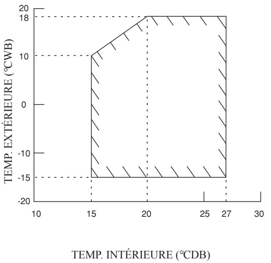
CHAUFFAGE
