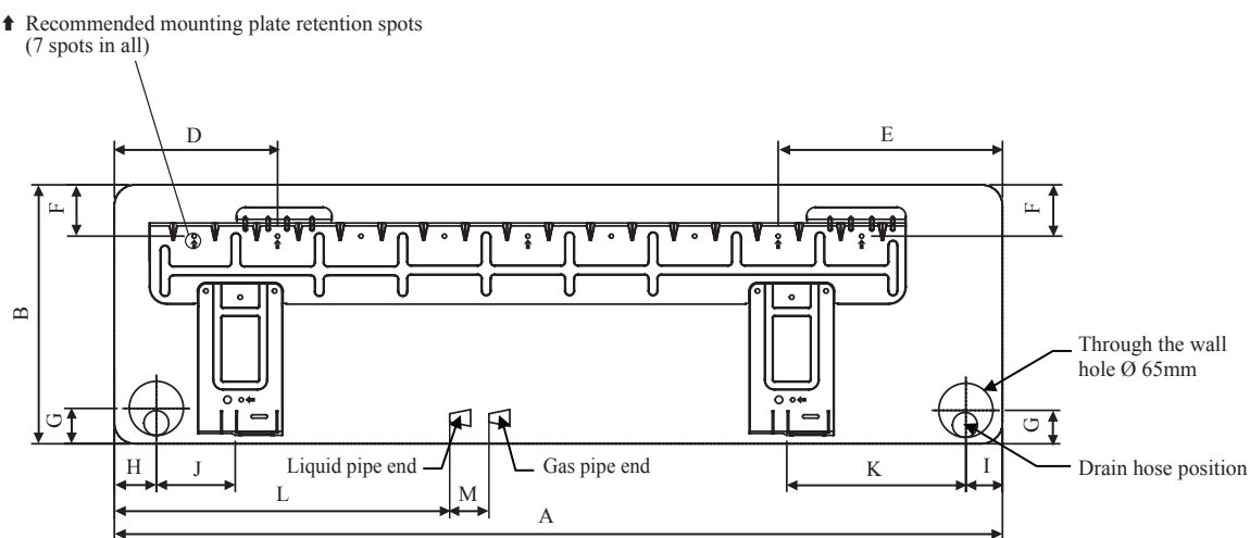
INSTALLATION PLATE 50/60
