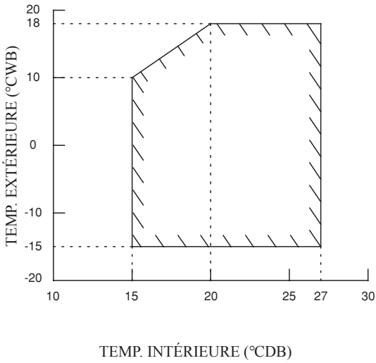
CHAUFFAGE
