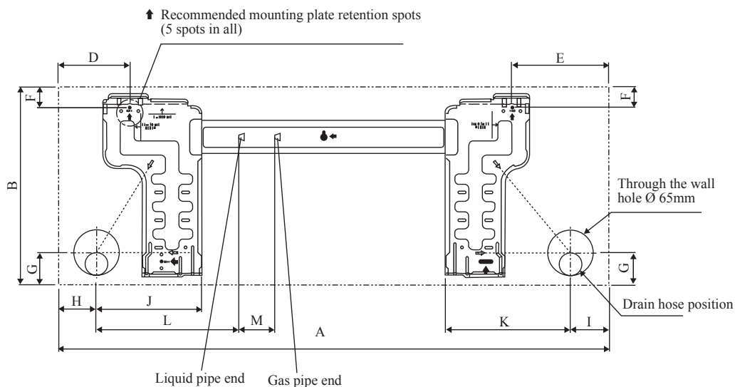
ALTERNATIVE INSTALLATION PLATE 25/35
