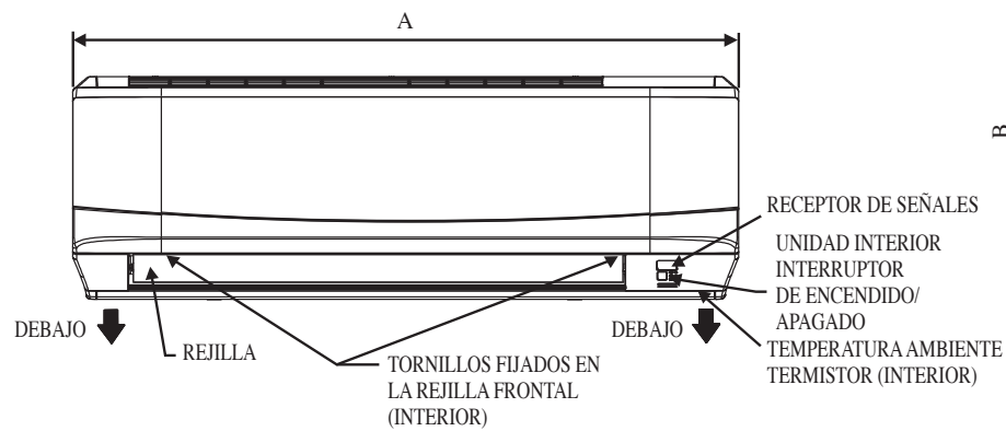
VISTA FRONTAL
